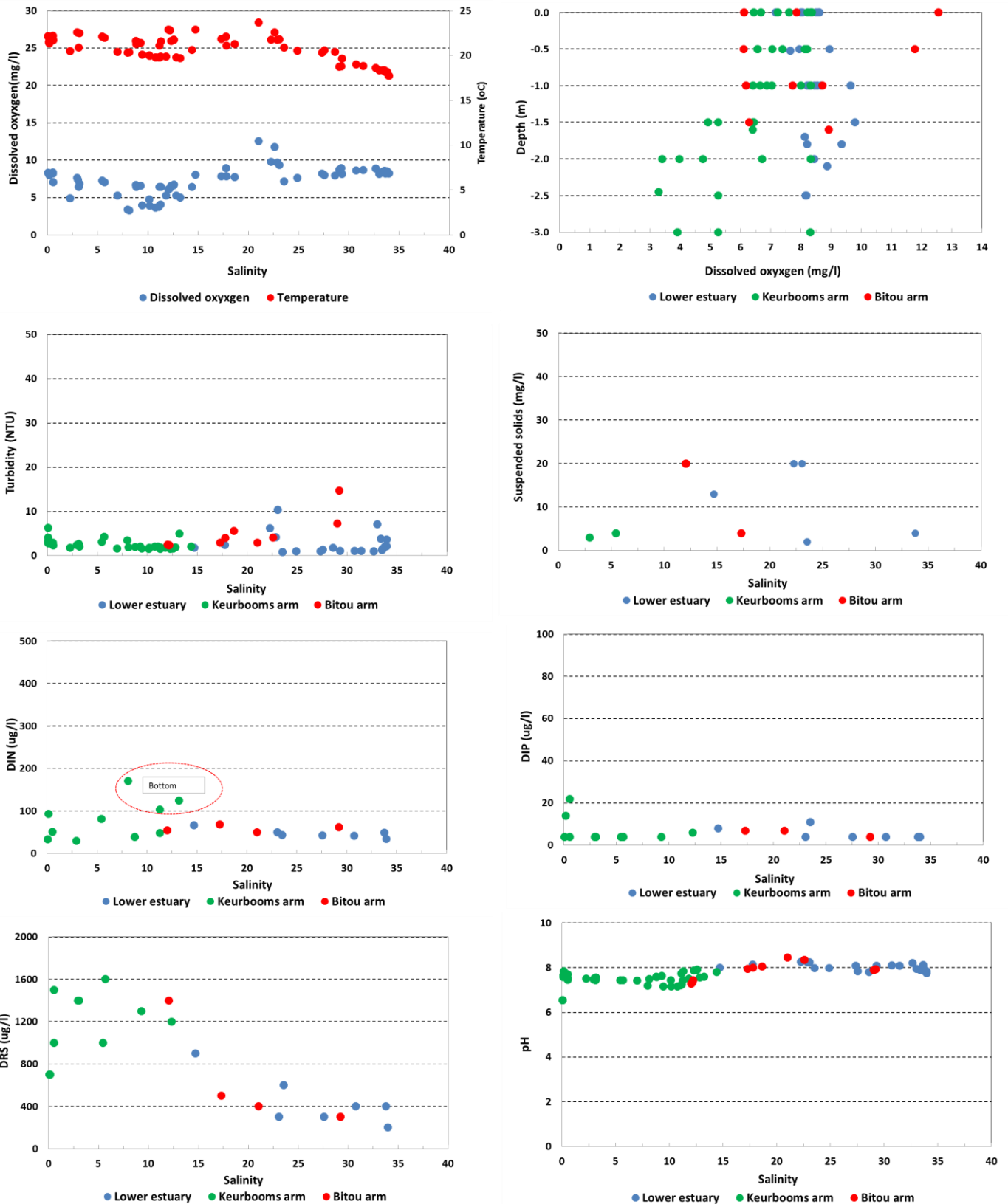
Figure A.2b Summary of water quality data collected in the Keurbooms Estuary on 9 December 2013
